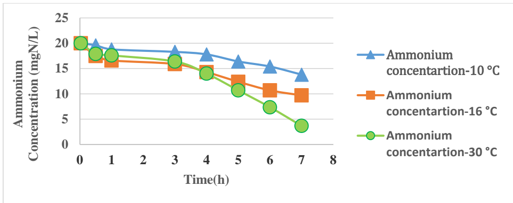
Figure 1.1 – The influence of increasing temperature on ammonium conversion rates at DO=0.5 mg/L
